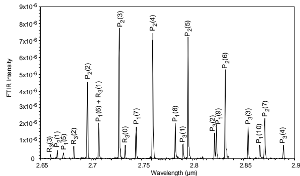
Figure 6. FTIR spectrum of HF(v,J) emission recorded in our HF production chamber. Spectral resolution is 0.5 cm -1 .
