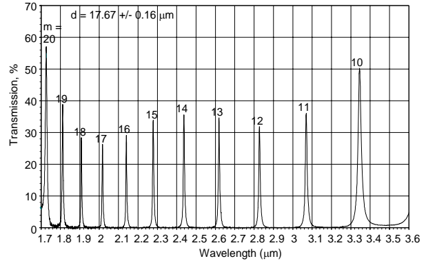
Figure 3. AIRIS transmission as a function of the wavelength of incident light for a mirror separation of 17.67 \pm 0.16 \mu\text{m} . The interference order is also indicated. Spectral resolution is 2 \text{cm}^{-1} .
