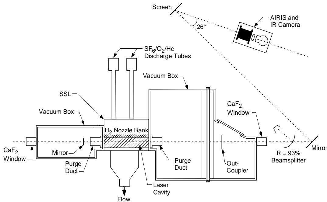
Figure 12. Optical setup for AIRIS spectral imaging measurements of projected SSL laser beam at UIUC.
