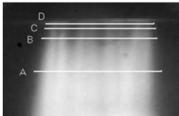
Figure 8. HF emission from P 2 (5) line. Analysis slices are indicated. Flow direction is down.
