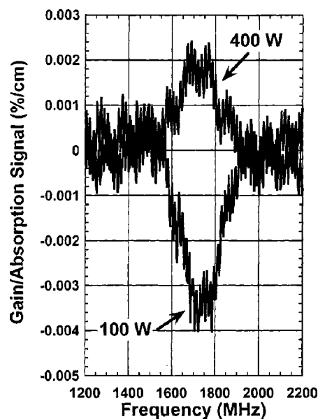
FIG. 2. Gain in the supersonic cavity as a function of frequency. Positive gain was observed at 400 W rf discharge power and absorption was observed at 100 W.
